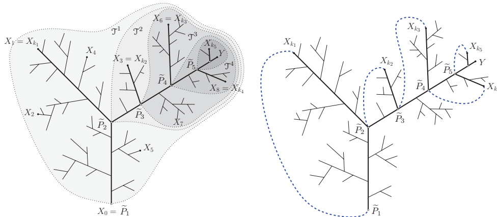
FIGURE 11. Illustration of the construction of \mathcal{T}^i for i \geq 0 and of the proof of Proposition 18.
